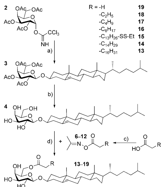
Scheme 1. Synthesis of acylated cholesteryl galactosides: a) 2 , cholesterol in \text{CH}_2\text{Cl}_2 (0.85 equiv), cat. TMSOTf, 1.5 h at RT, triethylamine, flash chromatography, 77%; b) 3 , MeOH, sodium methylate, pH 9–10, 3 h at RT, amberlite IR-120( \text{H}^+ ), flash chromatography, 54%; c) fatty acid, acetone oxime (1 equiv), EDC (1.25 equiv), cat. DMAP in \text{CH}_2\text{Cl}_2 , 2 h at RT, flash chromatography, 84–97%; d) 4 , fatty acid acetone oxime ester 6–12 (0.9 equiv), lipase Amano PS in pyridine, 10 days at 50°C, filtration, flash chromatography, 5–31%.
