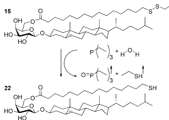
Scheme 4. Deprotection of the mercaptoethyl protecting group: 15 in pyridine/H 2 O 9:1, triethylphosphine (1 equiv) in THF, 30 min at RT, evaporation, 99 %.
