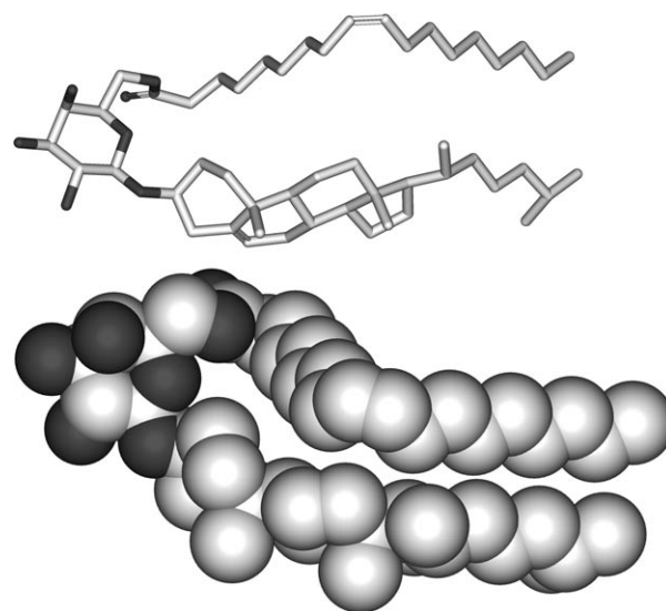
Figure 4. Structural depiction of ACGal C18:1: Representation as a capped sticks (top) and a space filled model (bottom). Built and minimized by using Sybyl 7.0. First Steepest descent then a conjugate gradient until a gradient of 0.05 kcal mol -1 Å -1 was reached for each routine.
