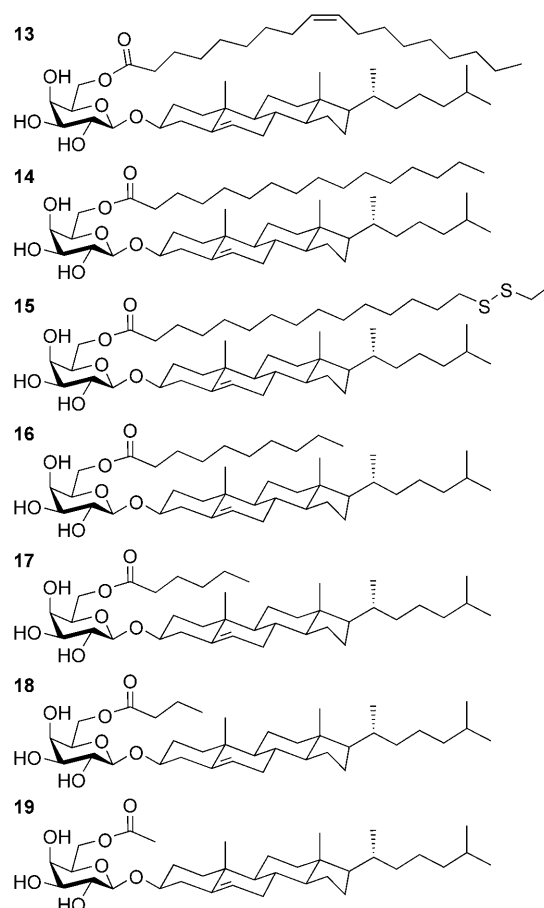
Scheme 2. Synthesized acylated cholesteryl galactosides: The glycolipid library consists of seven ACGal derivatives with a varying FA chain length from C 18:1 to C 2.
