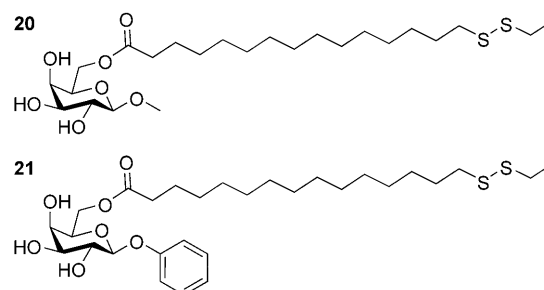
Scheme 3. Synthesized acylated non-cholesteryl galactosides: Two 6- O -acylated galactosides were synthesized that contain methyl or phenyl groups as a replacement for cholesterol.
